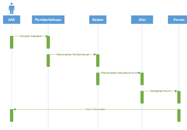
Gambar 3. 27 Sequence Tim Ahli
