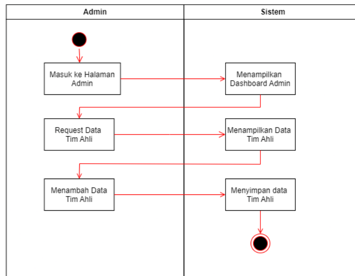
Gambar 3. 4 Activity Admin Tim Ahli Tambah
