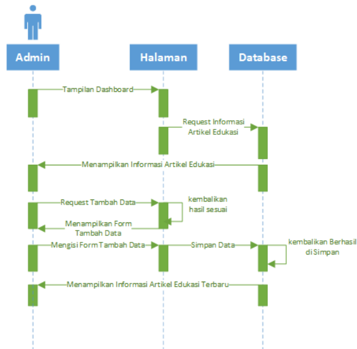
Gambar 3. 19 Sequence Admin Tambah Edukasi
