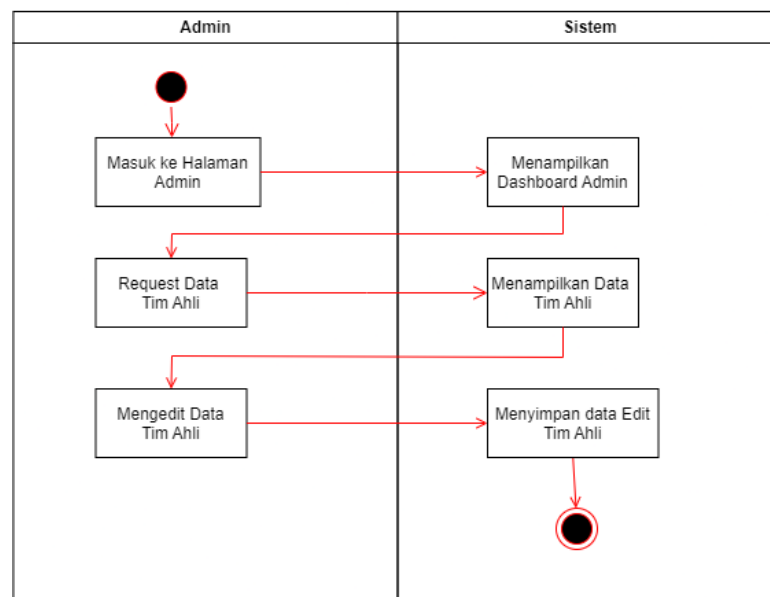
Gambar 3. 5 Activity Admin Tim Ahli Edit
