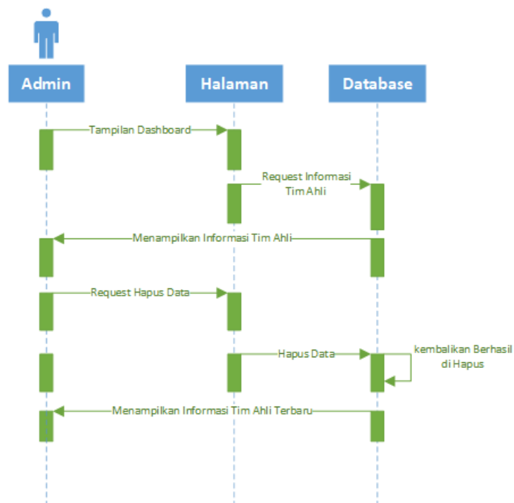
Gambar 3. 26 Admin Hapus Data Tim Ahli
