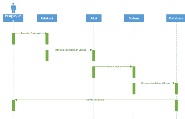
Gambar 3. 29 Sequence Edukasi
