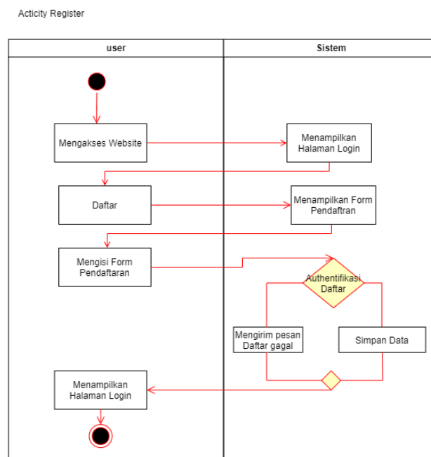
Gambar 3. 3 Activity Register
