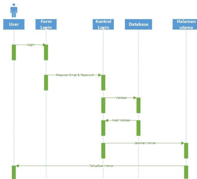
Gambar 3. 18 Sequence Login
