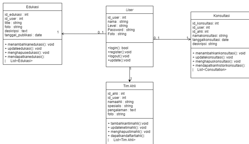
Gambar 3. 32 Class Diagram
