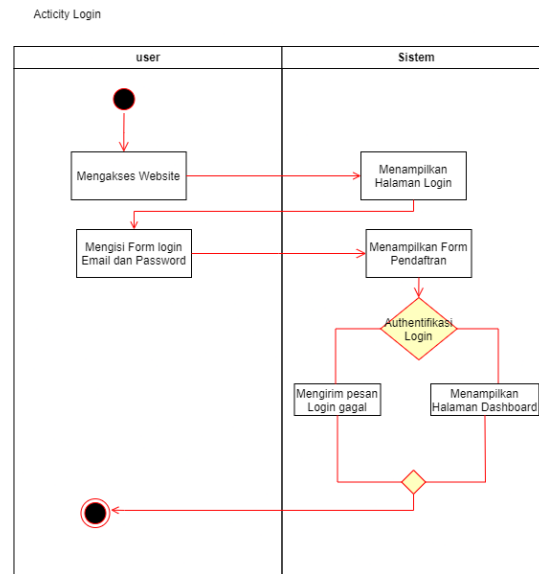
Gambar 3. 2 Activity Login
