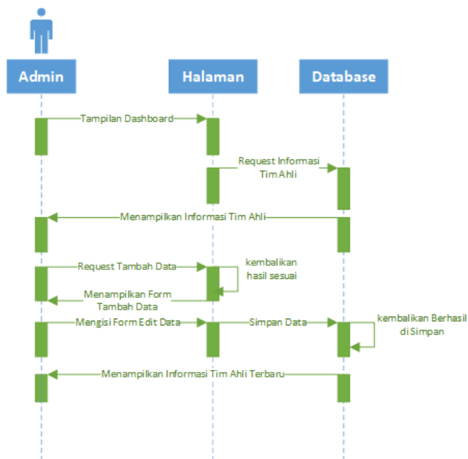
Gambar 3. 24 Sequence Admin Tim Ahli
