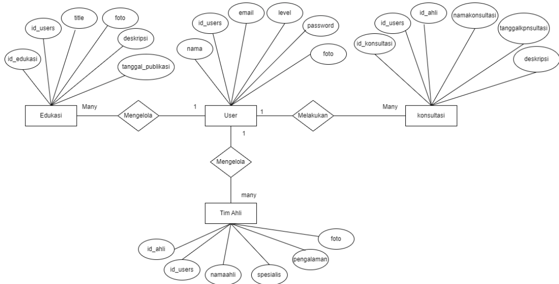
Gambar 3. 33 Entity Relationship Diagram
