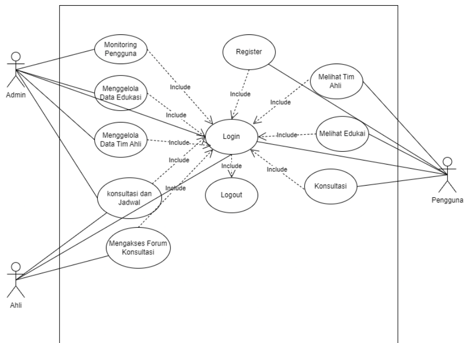
Gambar 3. 1 Use Case
