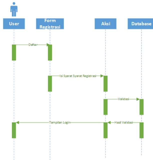
Gambar 3. 17 Sequence Registrasi
