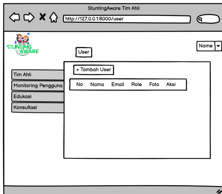
Gambar 3. 37 Monitoring User
